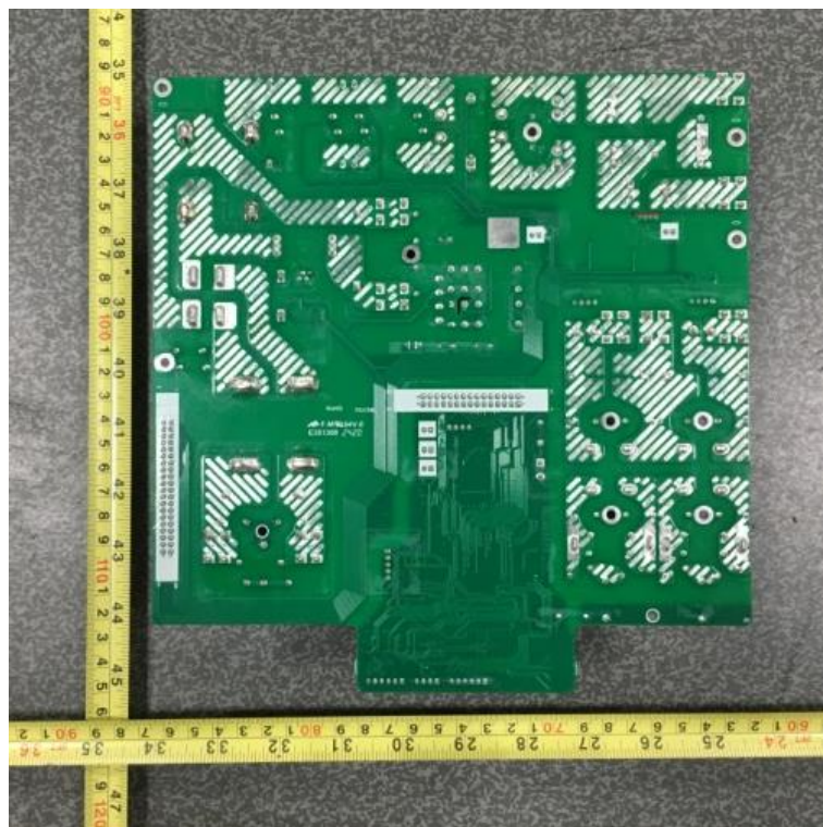
Input/output and connection board view (Soldered side)
