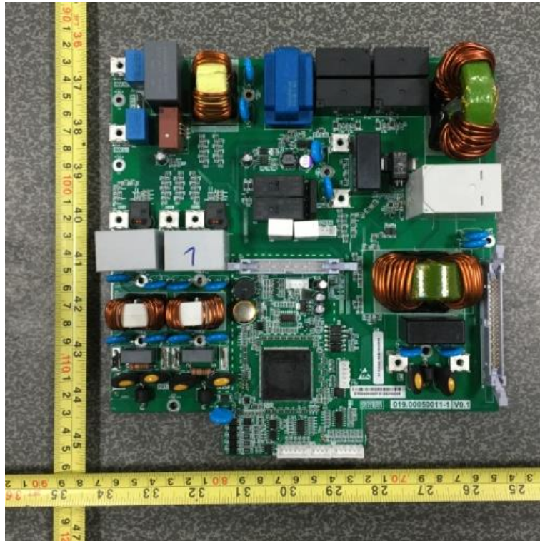
Input/output and connection board view (Components side)
