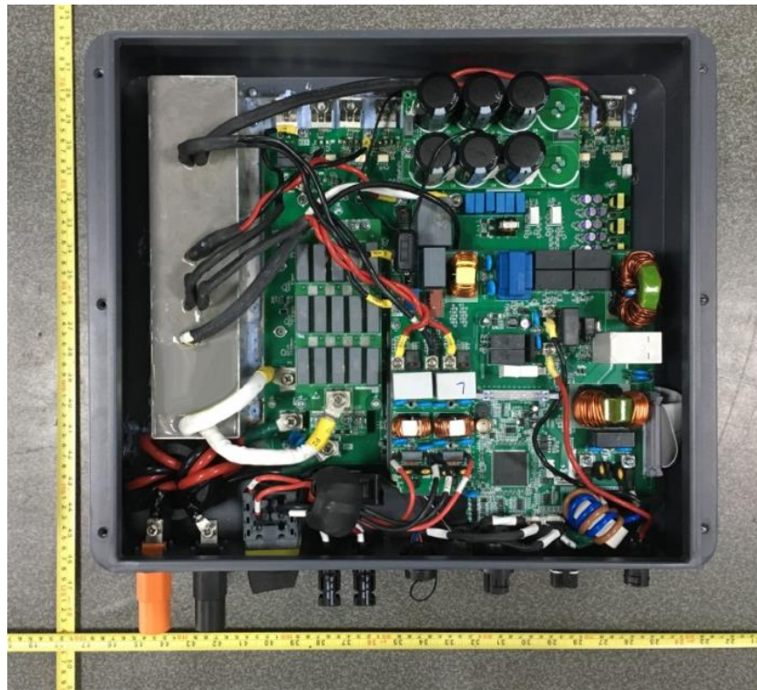
Internal view for model HYD 4000-EP, HYD 3600-EP, HYD 3000-EP
