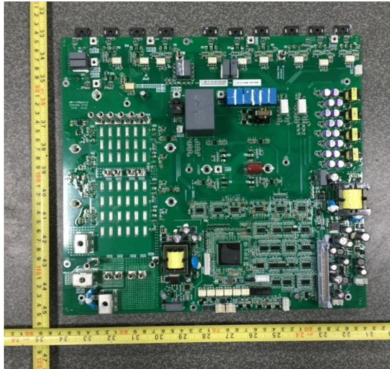
Power board view (Components side)
