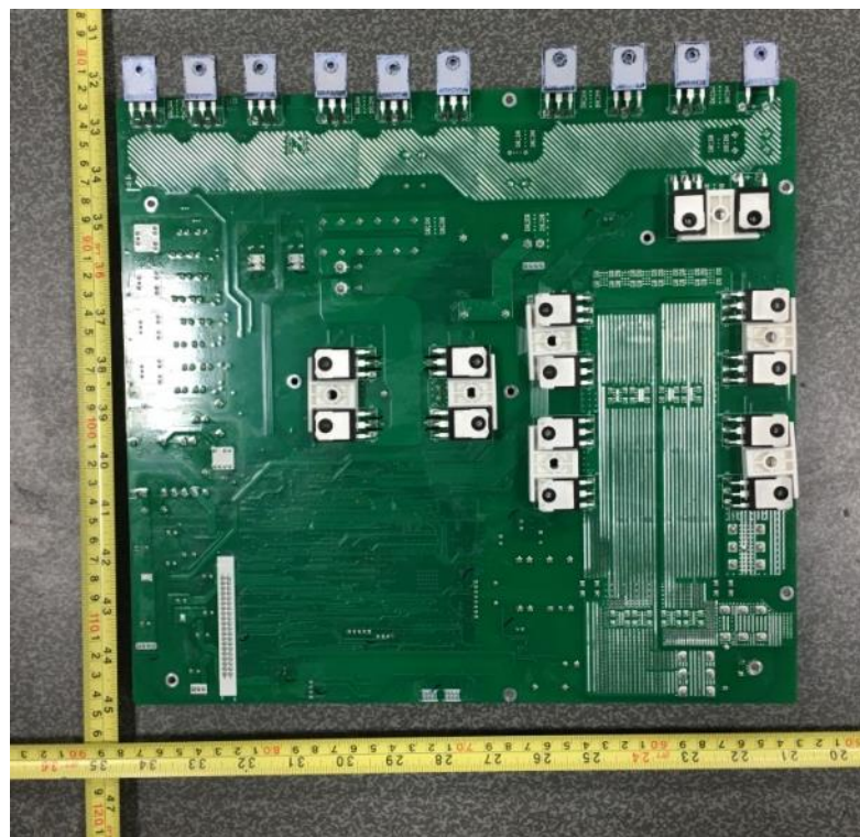
Power board view (Soldered side)
